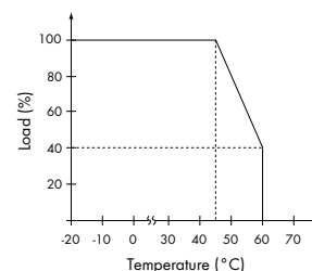
Fig. 6: Temperature derating curve
